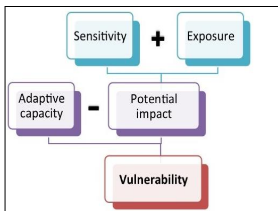
Figure 5: IPCC 2007 approach (Brugère et al., FAO 2015; Sharma et al., 2019)
